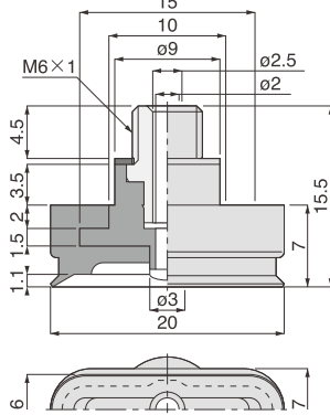
VP 6×20E□A
