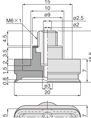
VP 5×20E□A
